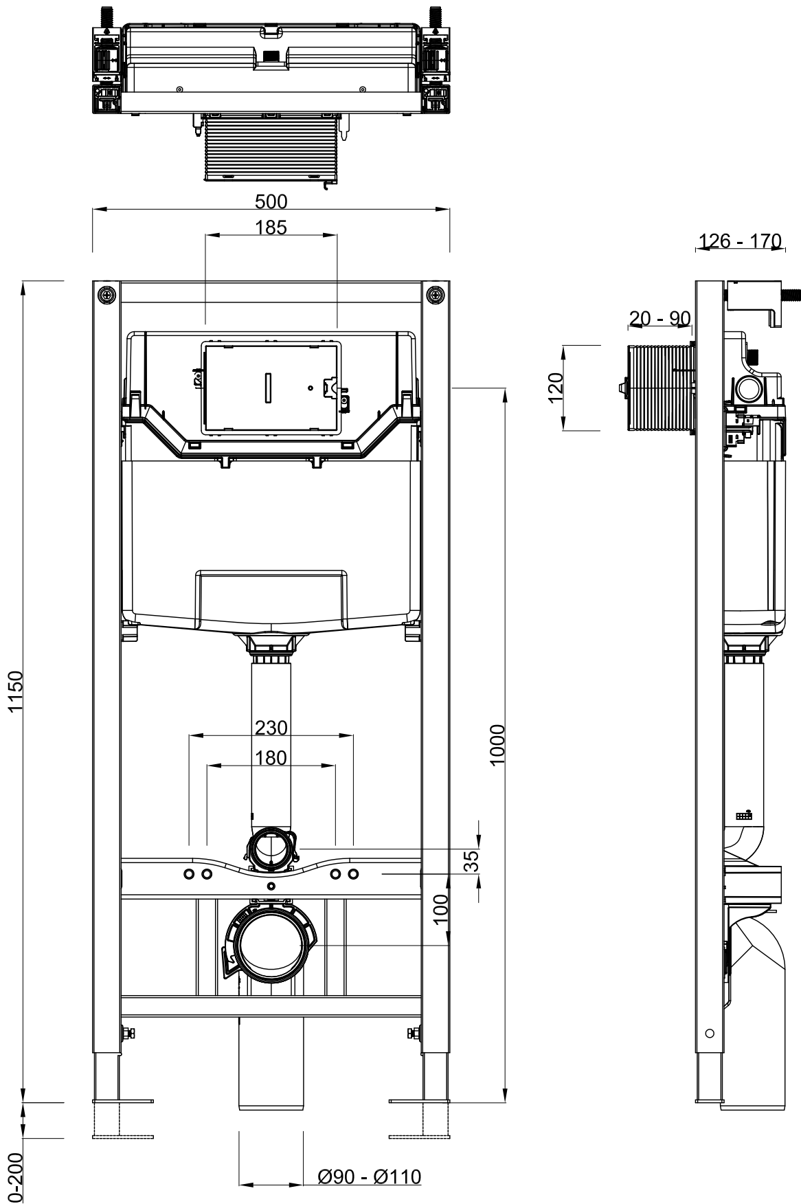
DOLPHIN SOLUTIONS LIMITED 126 PNEUMATIC CISTERN WITH 1150 FRAME DB5511.P
