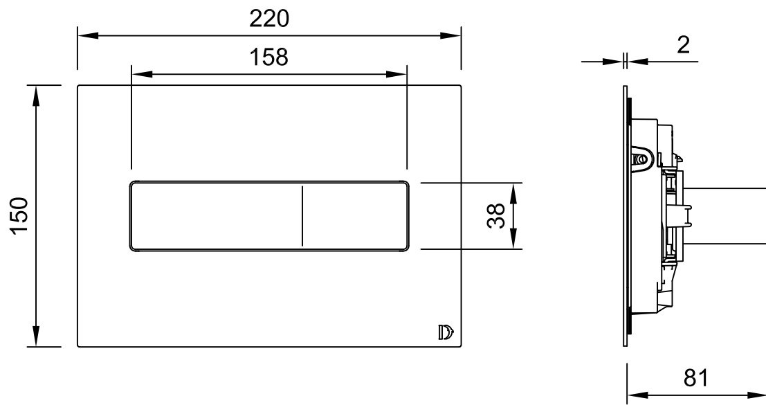
DOLPHIN SOLUTIONS LIMITED PNEUMATIC WC FLUSH PLATE DB5550.P
